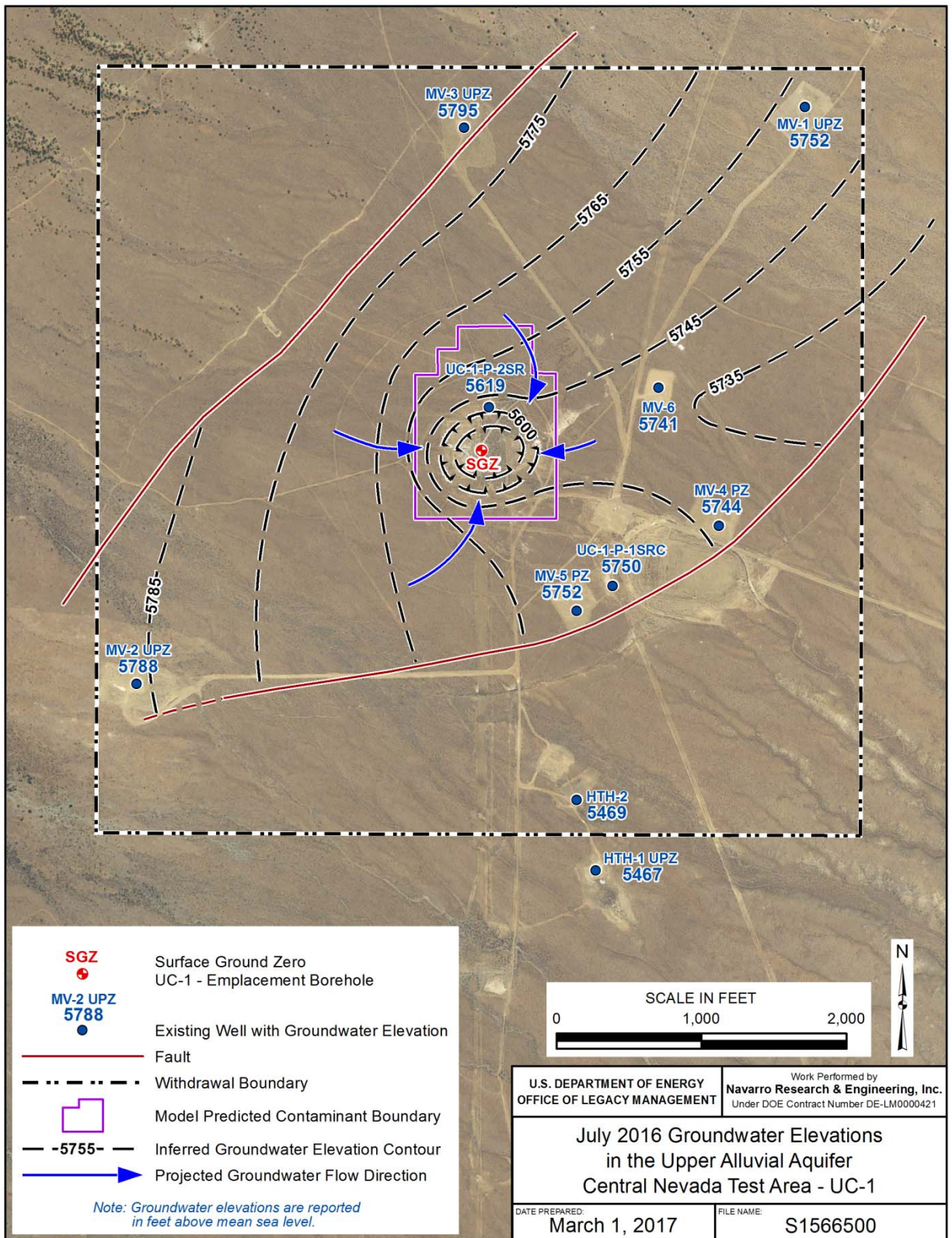
Figure 10. July 2016 Groundwater Elevations in the Upper Alluvial Aquifer CNTA—UC-1
