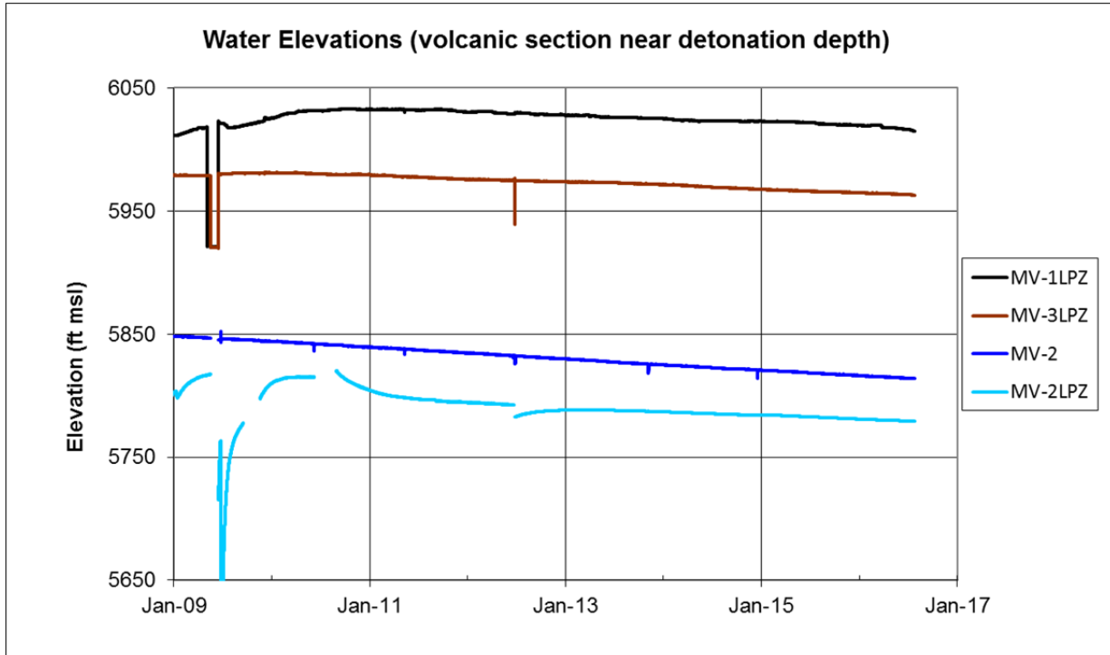
Figure 8. Water Elevations for the Well and Piezometers Screened in the Volcanic Section at or near the Depth of the Detonation
