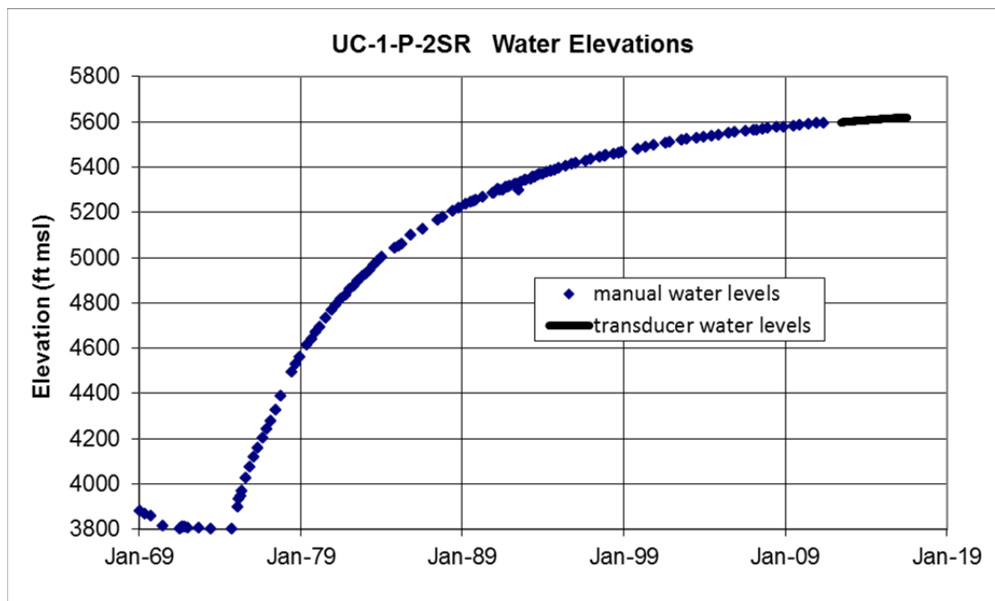
Figure 5. Water Elevations in Reentry Well UC-1-P-2SR http://nevada.usgs.gov/doe_nv/sitepage_temp.cfm?site_id=383806116125951
