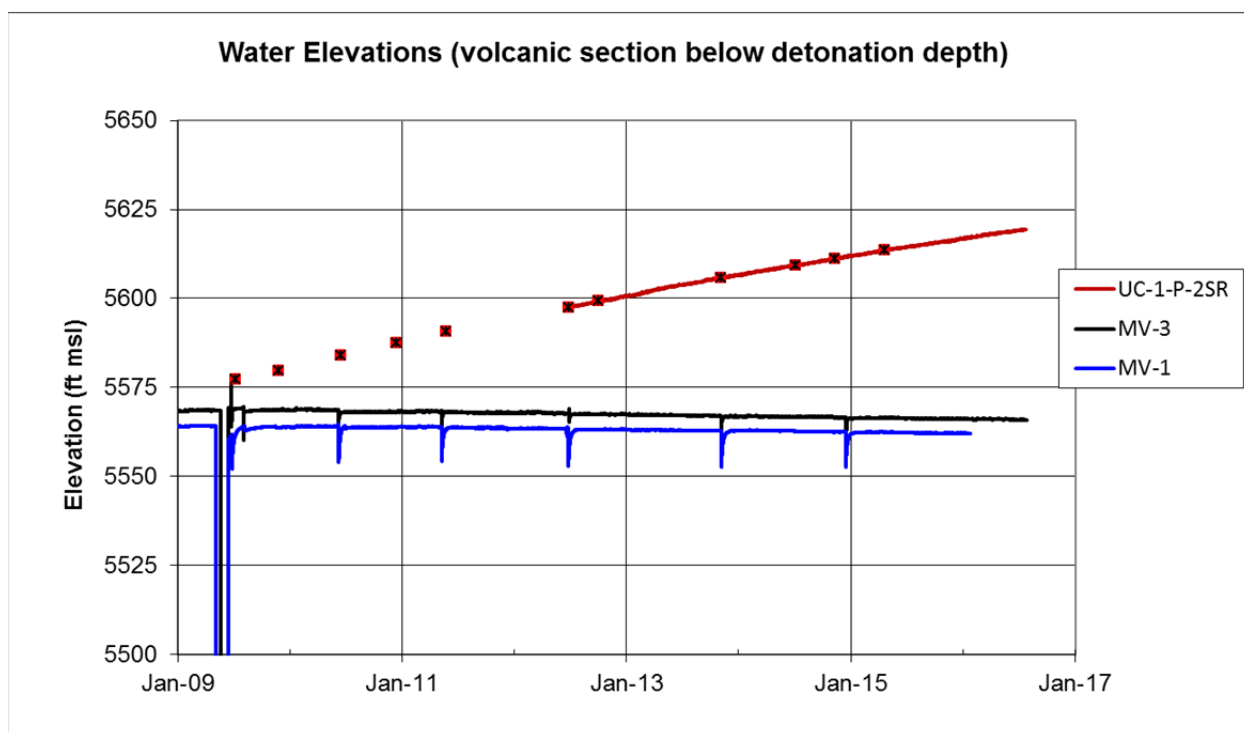
Figure 9. Water Elevations for the Wells Screened in the Volcanic Section Below the Depth of the Detonation (Water elevations for reentry well UC-1-P-2SR [drilled into the chimney] are shown for reference.)
