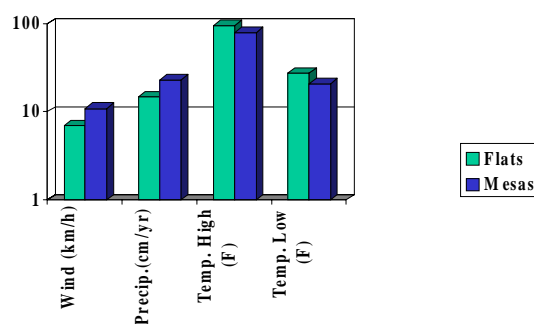
NTS METEOROLOGY
