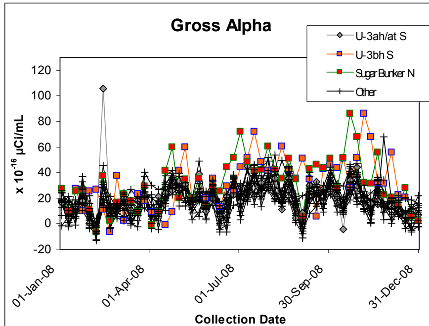
Figure 3-11. Gross alpha radioactivity in air samples collected in 2008
